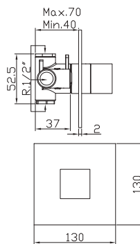
Concealed shower
