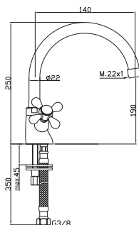
Basin Mixer
