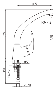
Sink mixer
