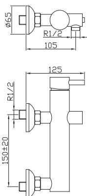
Shower mixer
