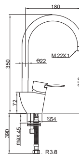
Sink mixer
