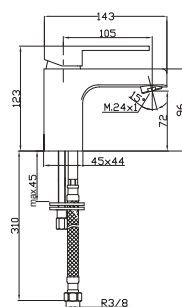
Basin mixer
