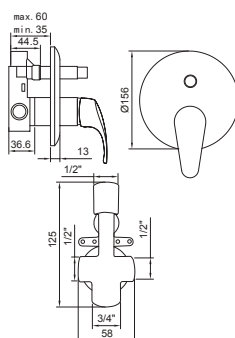
Concealed bath-shower
