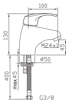
Basin mixer
