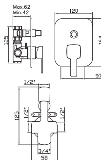
Concealed bath-shower
