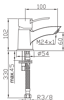
Basin mixer
