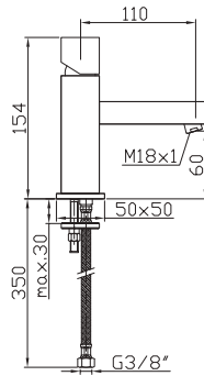
Basin mixer
