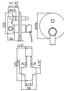
Concealed bath-shower
