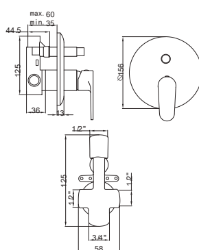
Concealed bath-shower
