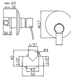
Concealed shower
