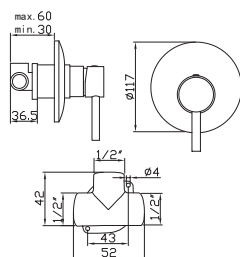
Concealed bath-shower
