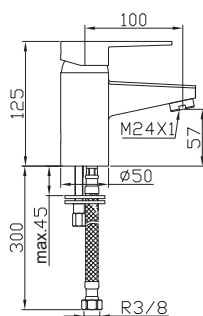
Basin mixer
