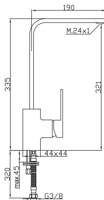
Sink Mixer
