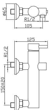
Shower mixer
