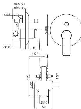
Concealed bath-shower
