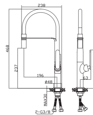
F8 MONOMANDO FREG.EXTRAÍBLE FLEXIBLE REF. 65808 / 65808-Sline
