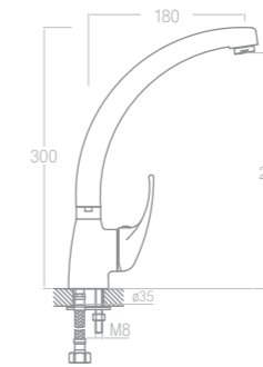
MONOMANDO FREGADERA V. TIERRA FRANCIA REF. 65807
