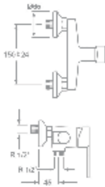
MONOMANDO DUCHA REF. 68084
