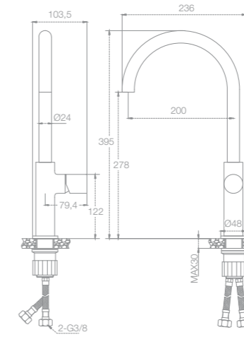
MONOMANDO FREGADERA REF. 68195 / 68195-Sline
