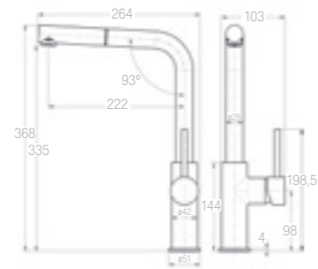
F20 MONOMANDO FREGADERA EXTRAÍBLE REF. 65820
