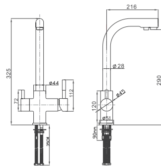
F13 MONOMANDO FREGADERA OSMOSIS CENTURY (2 MANETAS) REF. 65813
