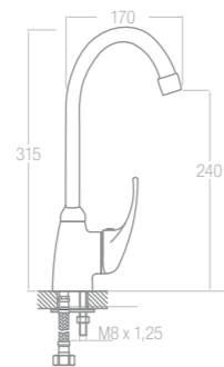
OASIS MONOMANDO FREGADERA "ECO" VERTICAL REF. 65817
