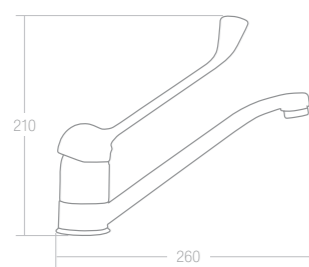
MEDICAL MONOMANDO FREGADERA HORIZONTAL REF. 14053
