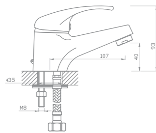
MONOMANDO LAVABO REF. 68011
