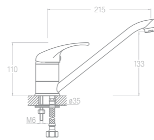
OASIS MONOMANDO FREGADERA HORIZONTAL REF. 68017
