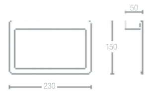
TOALLERO ANILLA CROMO REF. 30621
