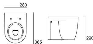
Tampo . Tapa . Cover . Abbatant 50259XX0 [CM]
